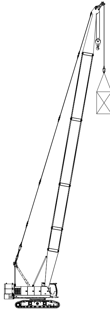
HC Configuration (double hooks, load on aux. hook)
