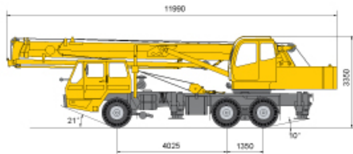
▲ Outline dimensions
