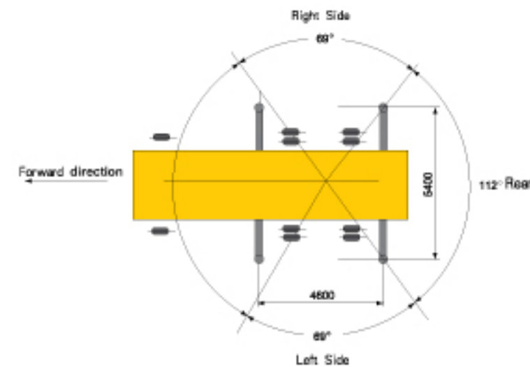
▲ Working Area
