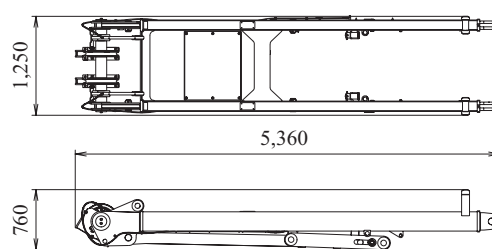
Gantry Weight: 1,320 kg
