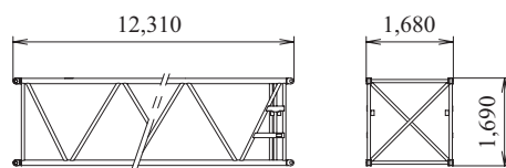
12.2 m Boom insert Weight: 1,195 kg
