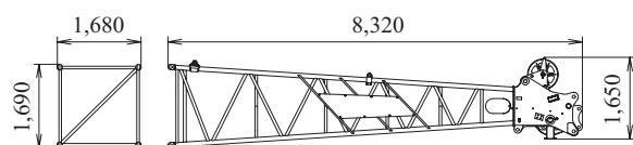
Boom tip Weight: 1,525 kg
