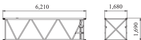
6.1 m Boom insert Weight: 655 kg
