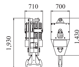
110 t hook Weight: 1,700 kg
