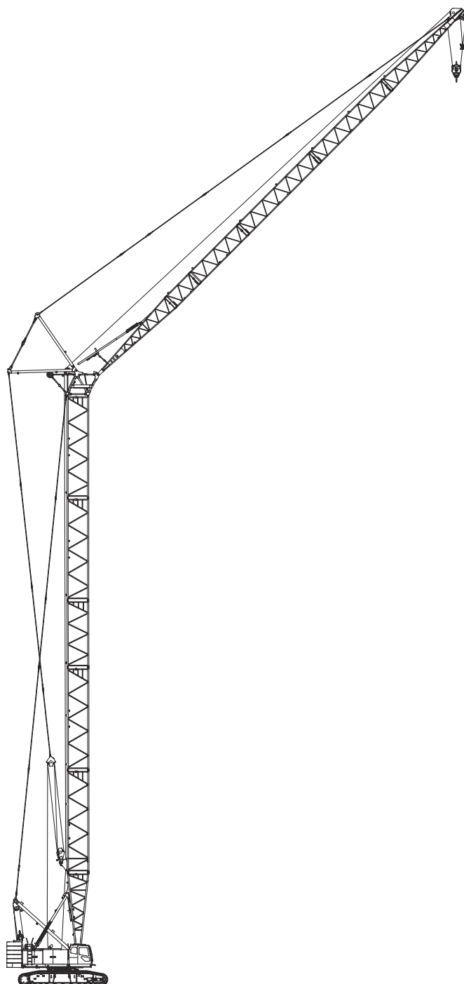
Tower Specification (Tower + Tower Jib Longest Length)
