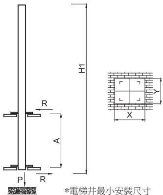
*電梯井最小安裝尺寸 Min.installation dimension of elevator shaft
