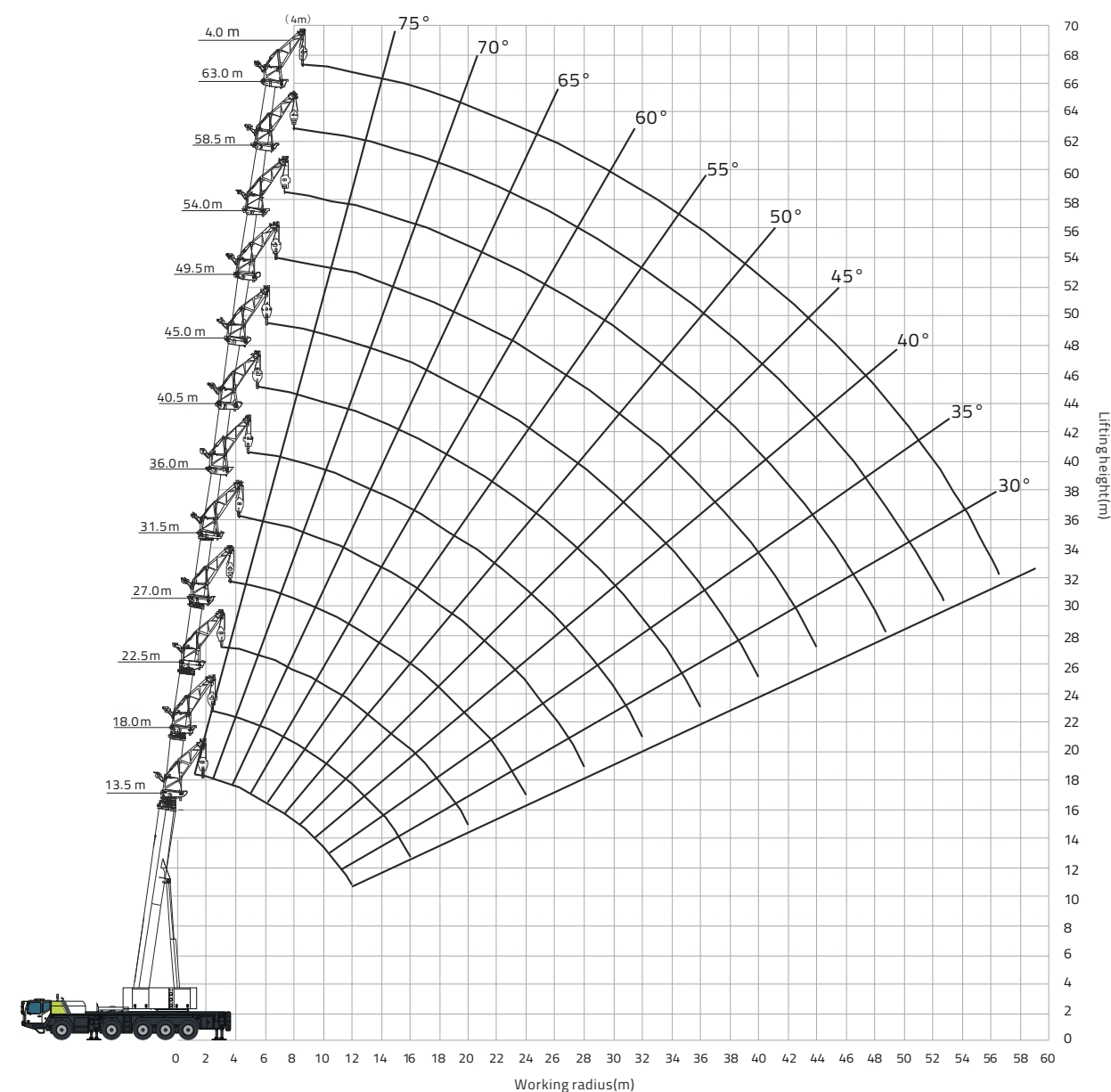
2.4.5 Main boom+ goose-head jib lifting height chart
