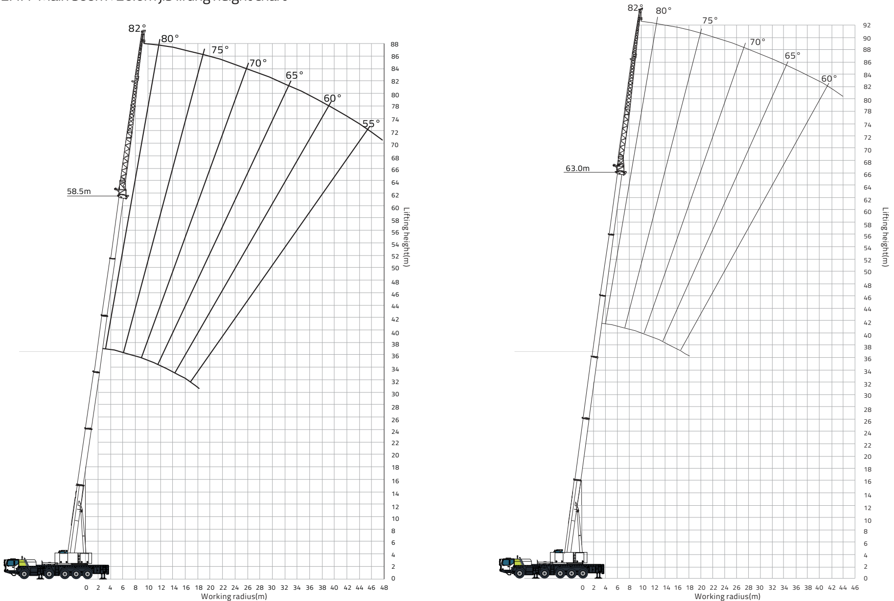
2.4.4 Main boom+26.6m jib lifting height chart
