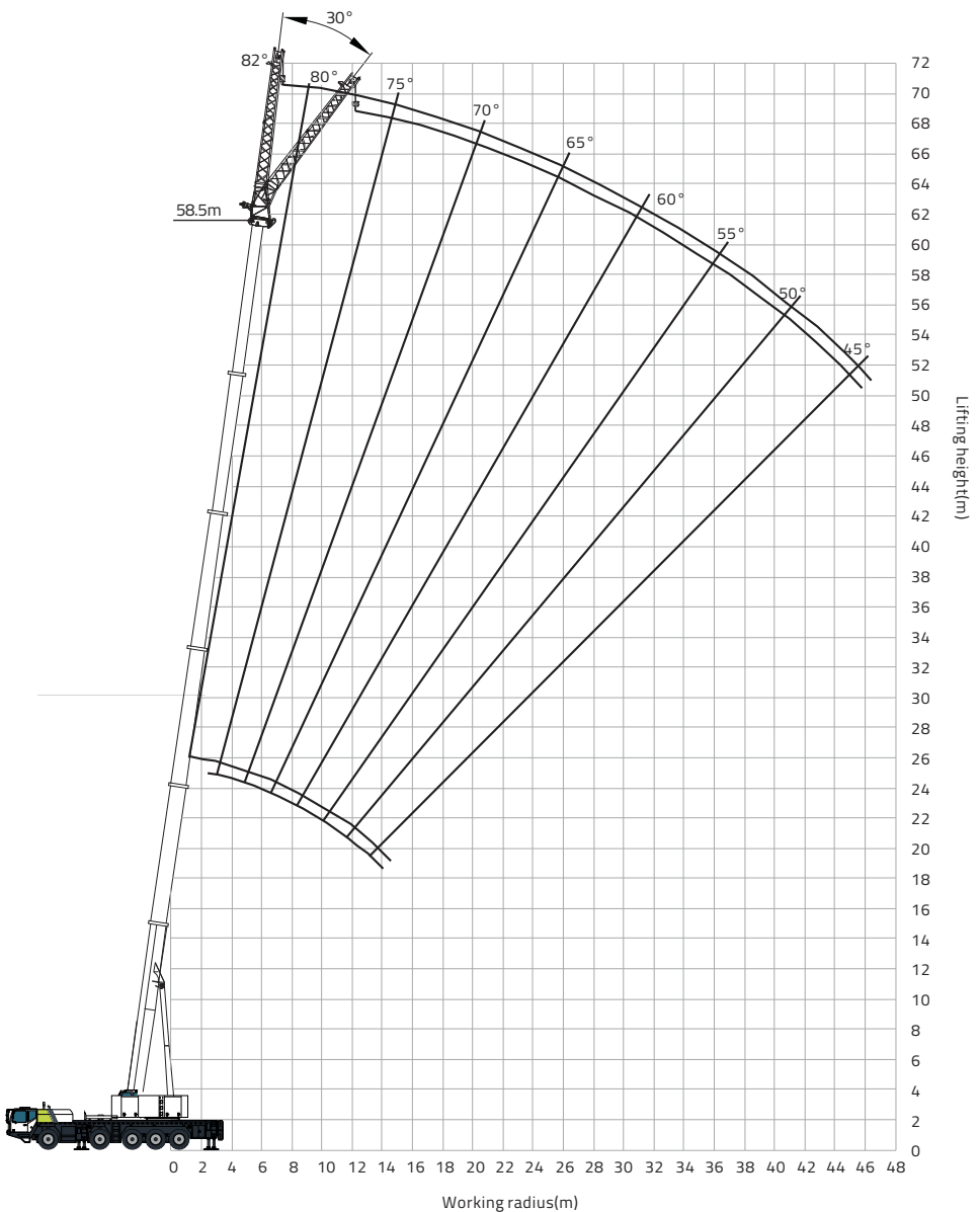
2.4.2 Main boom+11m jib lifting height chart
