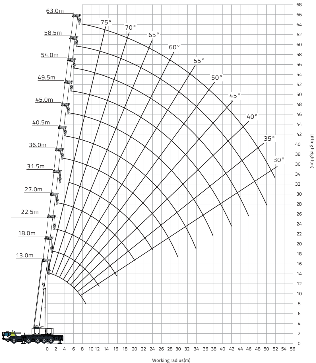
2.4.1 Main boom lifting height chart
